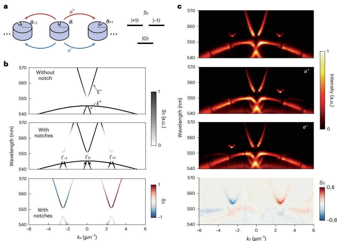
Fig. 2 | Spontaneous emission properties of perovskite metasurfaces.
