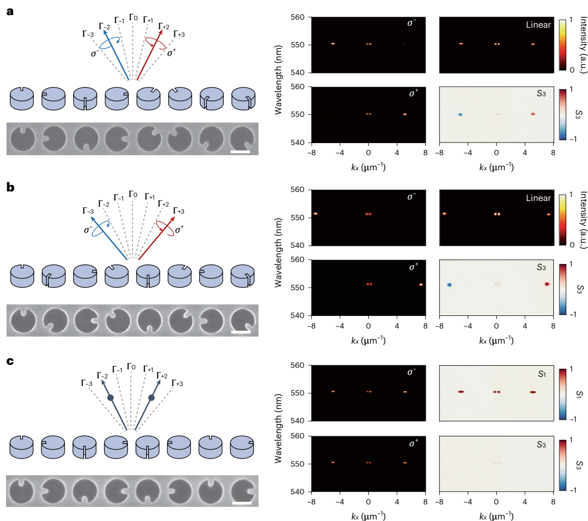
Fig. 4 | Perovskite lasing with tunable valleys and polarizations. a, b , Spin-valley-locked lasing at the \Gamma_{+2} valleys for W = 2 ( a ) and \Gamma_{+3} valleys for W = 3 ( b ). c , Linearly polarized lasing at the \Gamma_{+2} valleys for W = 0 . Angle- and polarization-resolved lasing spectra, as well as the corresponding Stokes parameters (right). Scale bars (SEM images), 200 nm.
