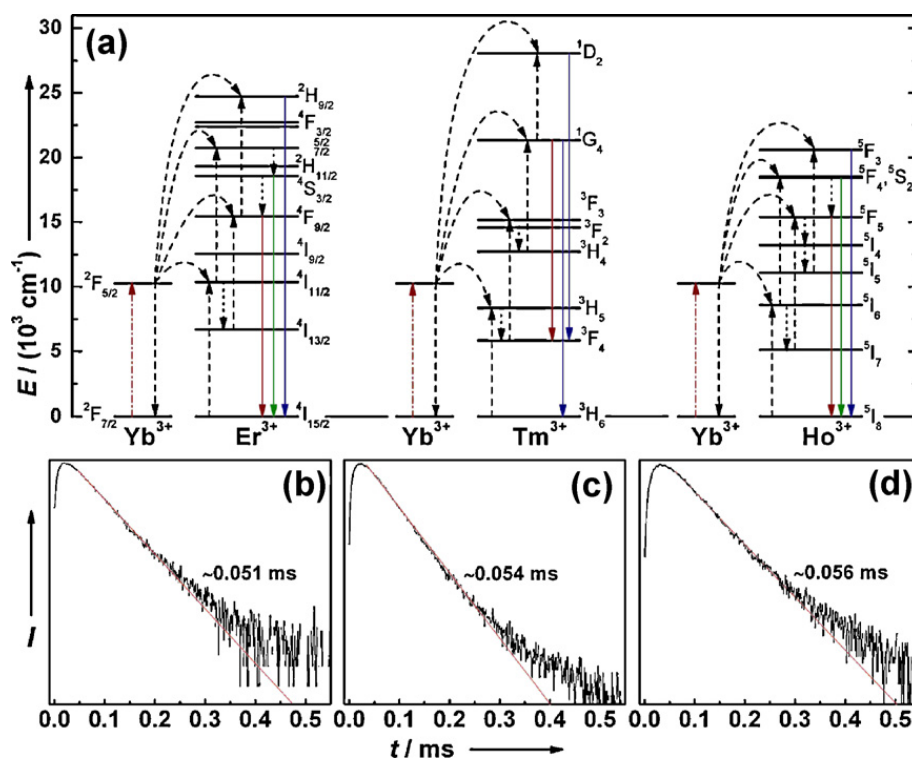
Fig. 4. (a) Schematic energy level diagrams showing typical UC processes for Yb 3+ , Er 3+ , Tm 3+ and Ho 3+ . The dashed-dotted, dotted, and full arrows represent excitation, multiphonon relaxation, and emission processes, respectively. (b–d) Luminescence decay curves of Er 3+ in LiYF 4 : Yb/Er (18/2 mol %) nanoparticles by monitoring the upconversion emission centered at 522 nm, 551 nm, and 669 nm. Flexible lines: experimental data; straight lines: fitting results by I(t) = I_0 \exp(-t/\tau) ( I_0 is the initial emission intensity at t = 0 , and \tau is the lifetime of the emission center).
