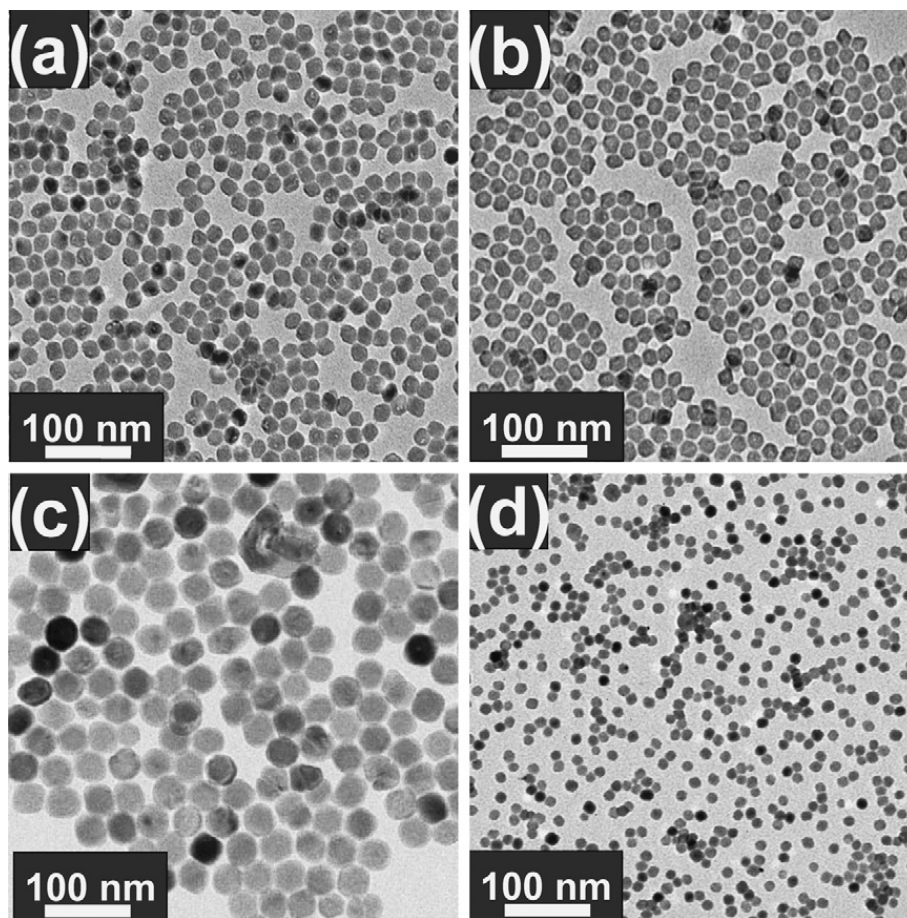
Fig. 2. TEM images of the as-synthesized nanoparticles with different doping compositions and metal-to-F ratios. (a) \text{LiYF}_4\text{:Yb/Ho} (18/2 mol %). (b) \text{LiYF}_4\text{:Yb/Tm} (20/0.2 mol %). (c) \text{LiYF}_4\text{:Yb/Er} (18/2 mol %) with a metal-to-F ratio of 3/8. (d) \text{LiYF}_4\text{:Yb/Er} with a metal-to-F ratio of 1/6.
