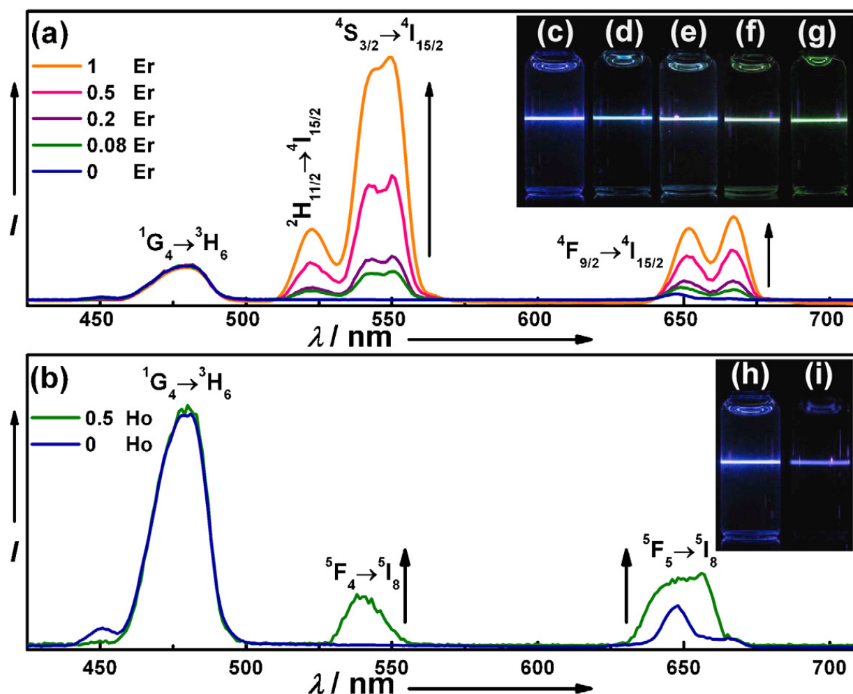
Fig. 5. Room temperature upconversion emission spectra of (a) LiYF_4:Yb/Tm/Er (20/0.2/0–1 mol %) and (b) LiYF_4:Yb/Tm/Ho (20/0.2/0–0.5 mol %) nanoparticles dispersed in cyclohexane solutions (8 mM). The spectra in (a) and (b) were normalized to Tm^{3+} 480 nm emission. (c–i) Compiled luminescent photos showing corresponding colloidal solutions of LiYF_4:Yb/Tm/Er (20/0.2/0–1 mol %) and LiYF_4:Yb/Tm/Ho (20/0.2/0–0.5 mol %), respectively.
