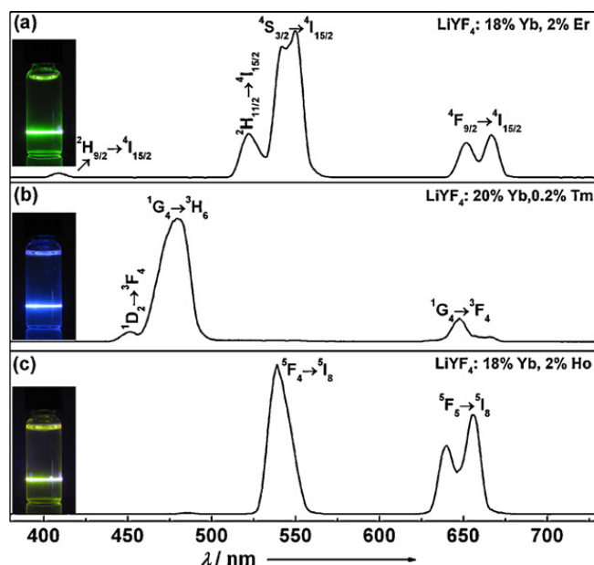
Fig. 3. Room-temperature upconversion emission spectra of LiYF 4 nanoparticles co-doped with (a) Yb/Er (18/2 mol %), (b) Yb/Tm (20/0.2 mol %), and (c) Yb/Ho (18/2 mol %). The samples were excited with a 980-nm diode laser operating at 600 mW. Inserts are digital camera photographs of corresponding solution samples.
