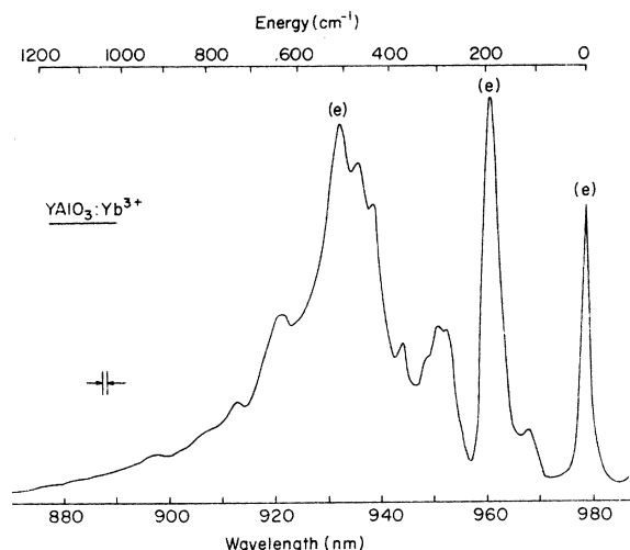
FIG. 3. Excitation spectrum of the ^2F_{5/2} \rightarrow ^2F_{7/2} fluorescence of \text{Yb}^{3+} in \text{YAlO}_3 at 77^\circ\text{K} . The three purely electronic transitions from the ground state are denoted by (e).
