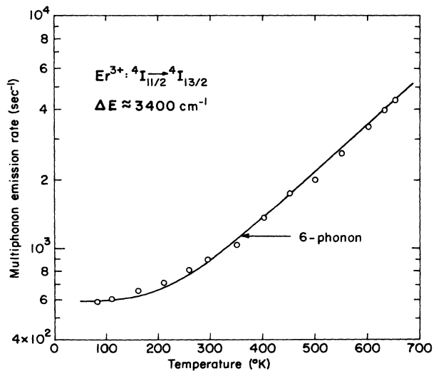
FIG. 6. Measured temperature dependence of the \text{Er}^{3+} {}^4I_{11/2} \rightarrow {}^4I_{13/2} multiphonon emission rate. The curve was calculated from Eq. (10) assuming relaxation by six 570- \text{cm}^{-1} phonons.
