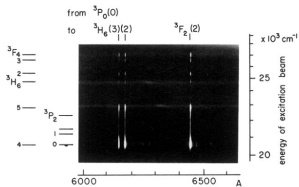
FIG. 2. Portion of the excitation survey plate taken at 4.2°K with a 100% \text{PrCl}_3 crystal. Any horizontal strip displays a fluorescence spectrum excited by the energy as marked on the right. Numbers in parentheses are the crystal quantum numbers of the respective Stark levels. Parts of two single-ion energy level diagrams are shown on the left to indicate the mechanism of excitation in a region with no single-ion levels.
