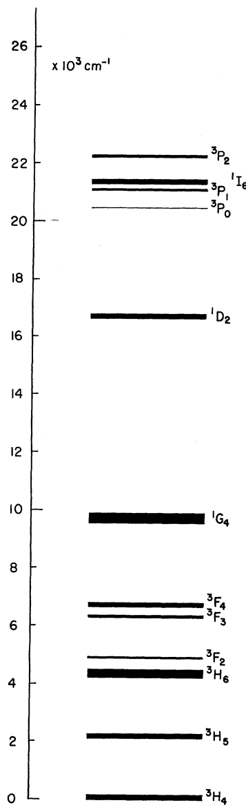
FIG. 1. Energy levels of \text{Pr}^{3+}(4f^2) . The width of the lines indicates the Stark splitting in a \text{LaCl}_3 crystal. The diagram is complete with the exception of one ^1S_0 level which is predicted above 50\,000\text{ cm}^{-1} by calculations.
